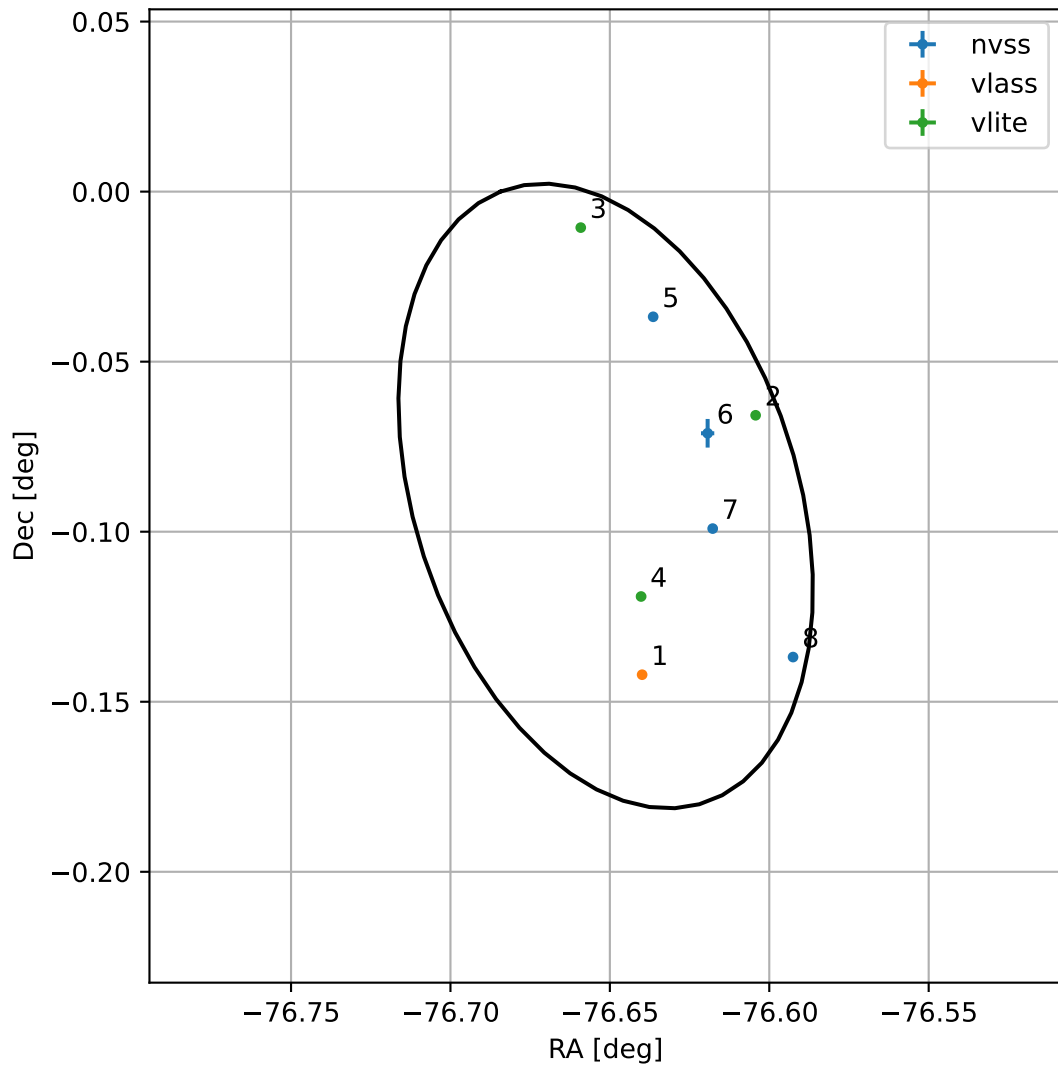
4FGL J1853.3-0005
