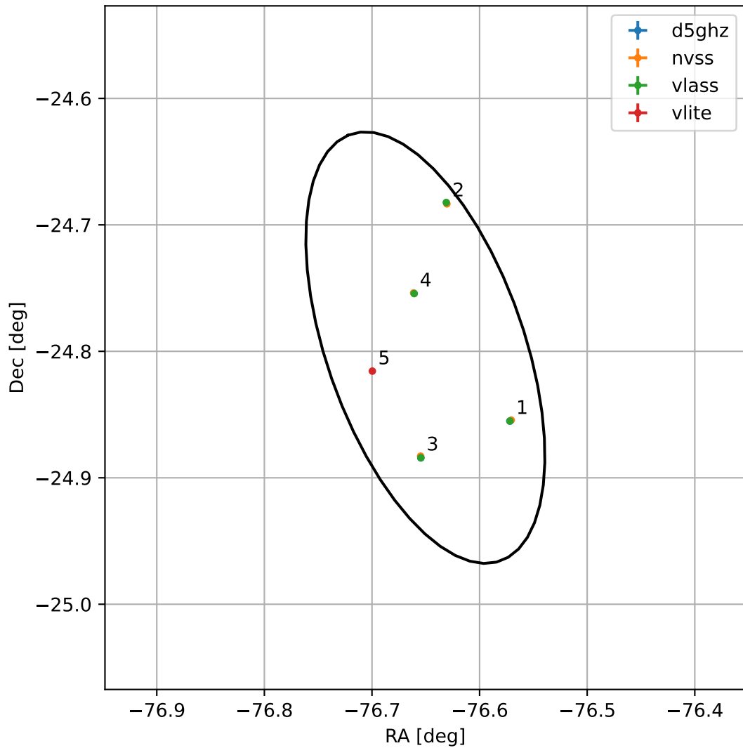
4FGL J1853.3-2447
