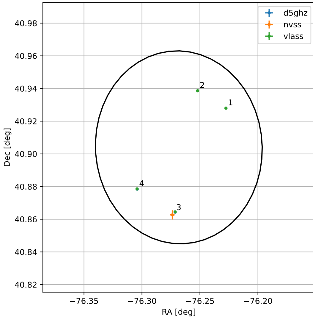
4FGL J1854.9+4054
