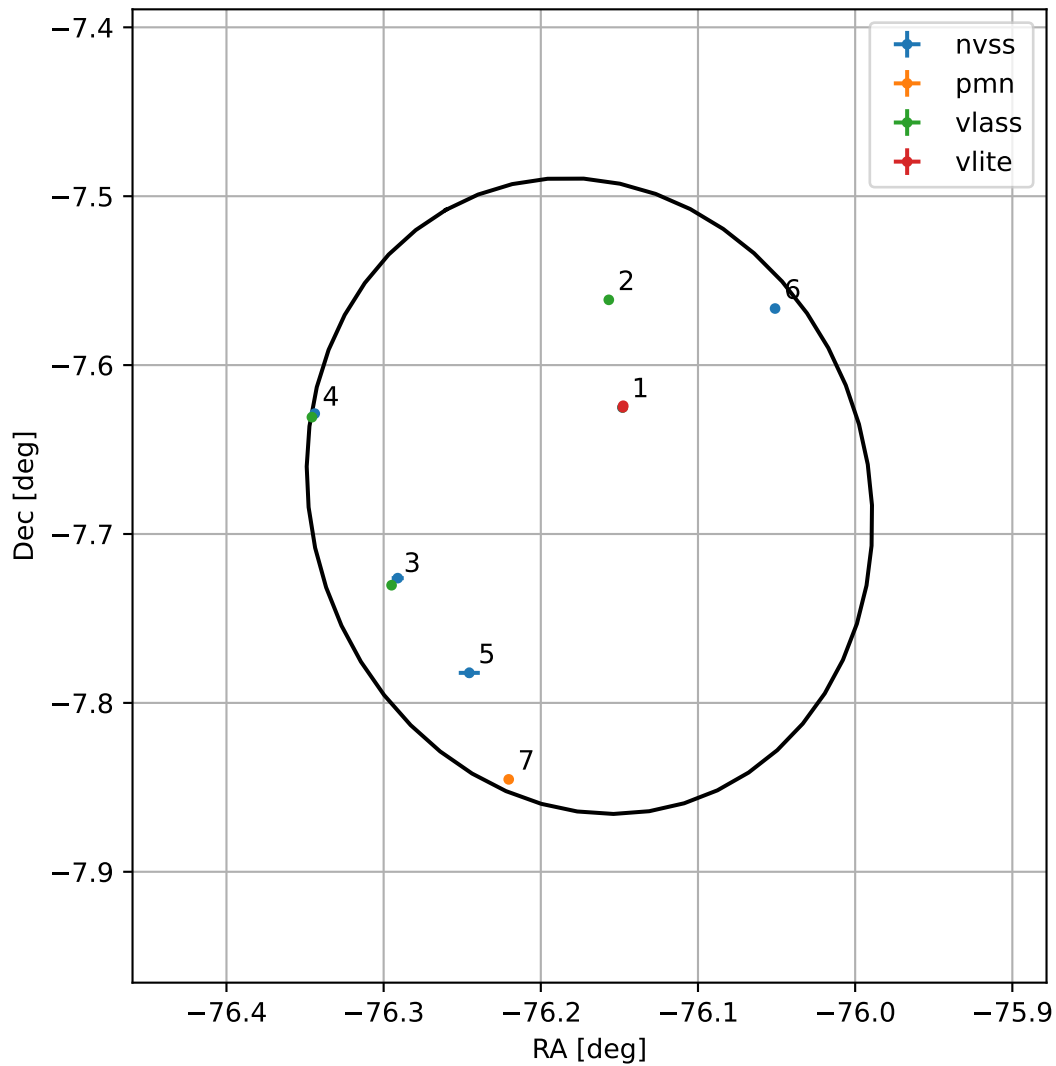
4FGL J1855.3-0740
