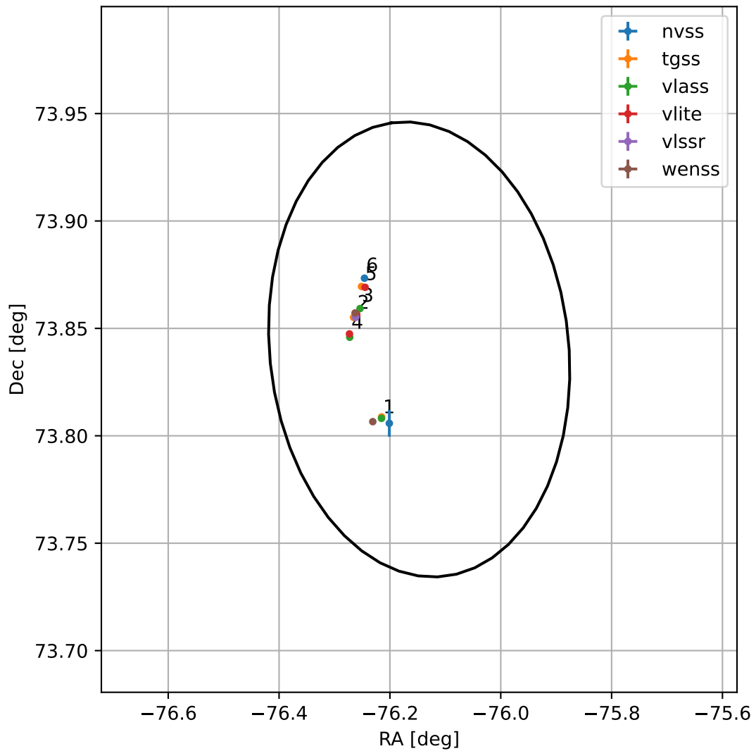
4FGL J1855.4+7350
