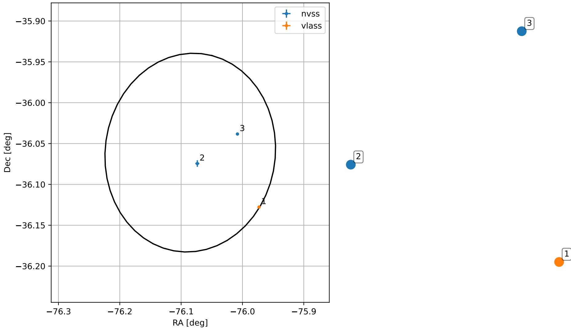
4FGL J1855.6-3603
