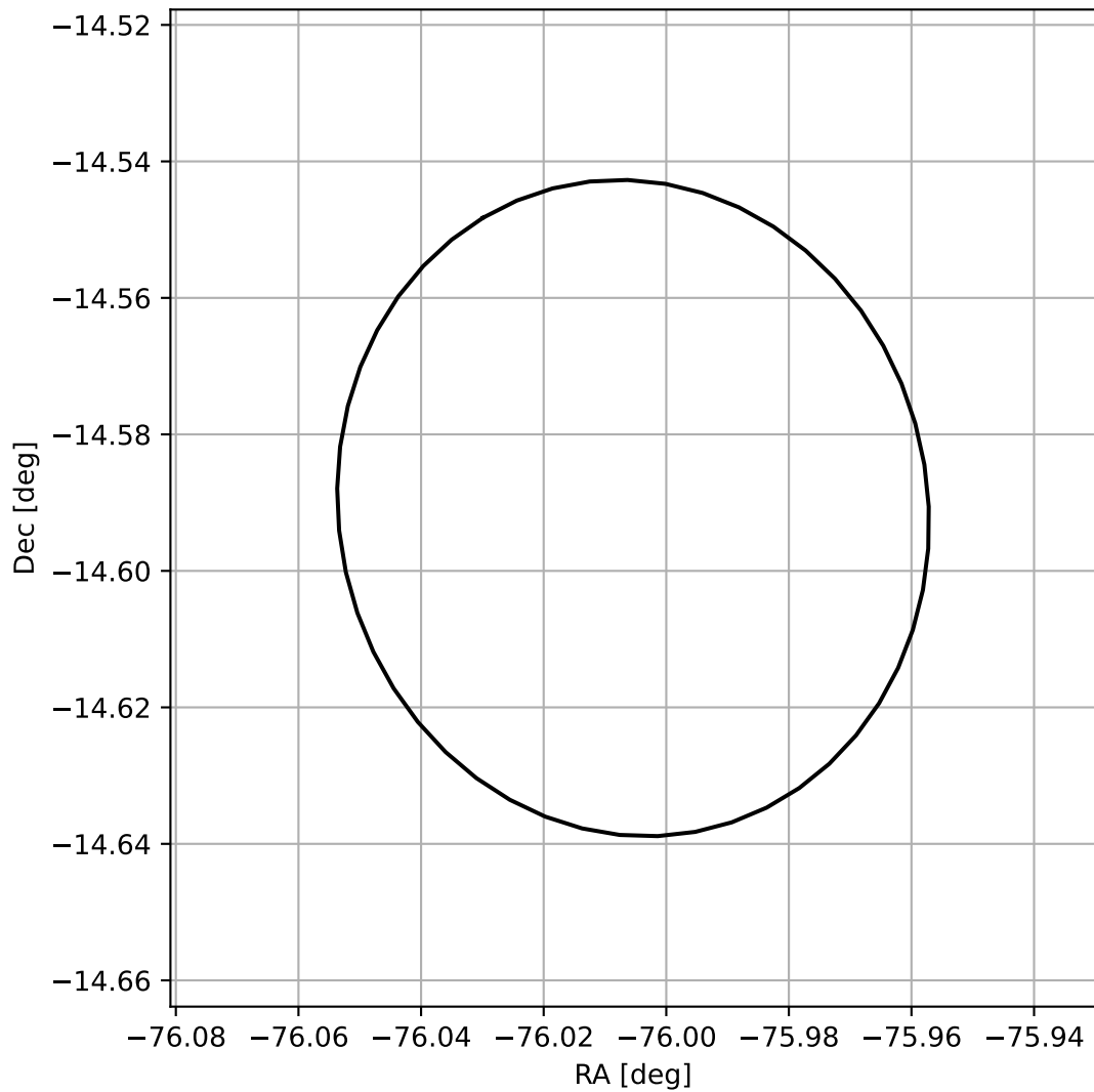
4FGL J1855.9-1435
