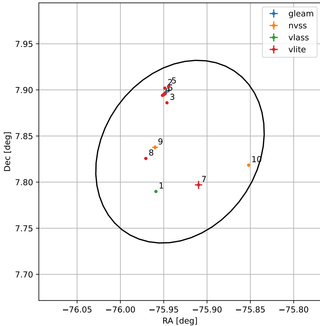
4FGL J1856.2+0749
