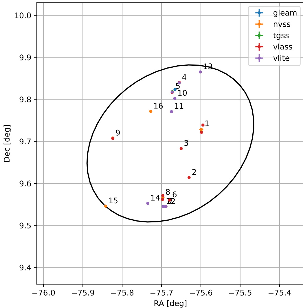
4FGL J1857.2+0941
