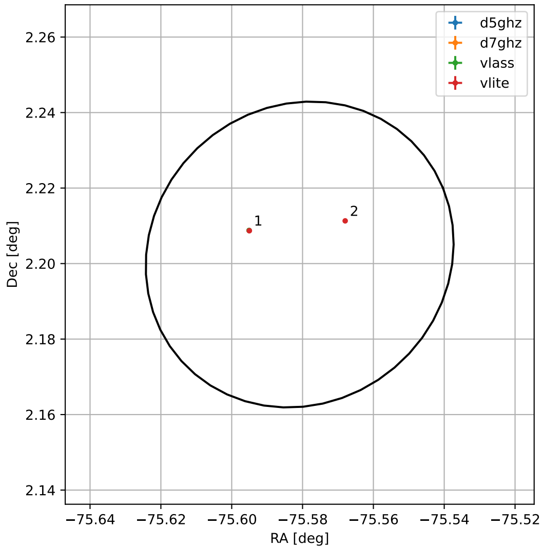
4FGL J1857.6+0212
