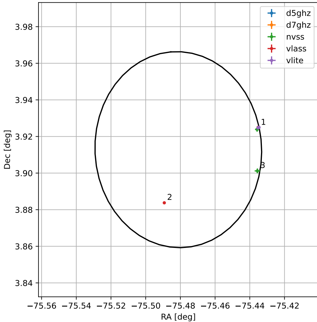
4FGL J1858.0+0354
