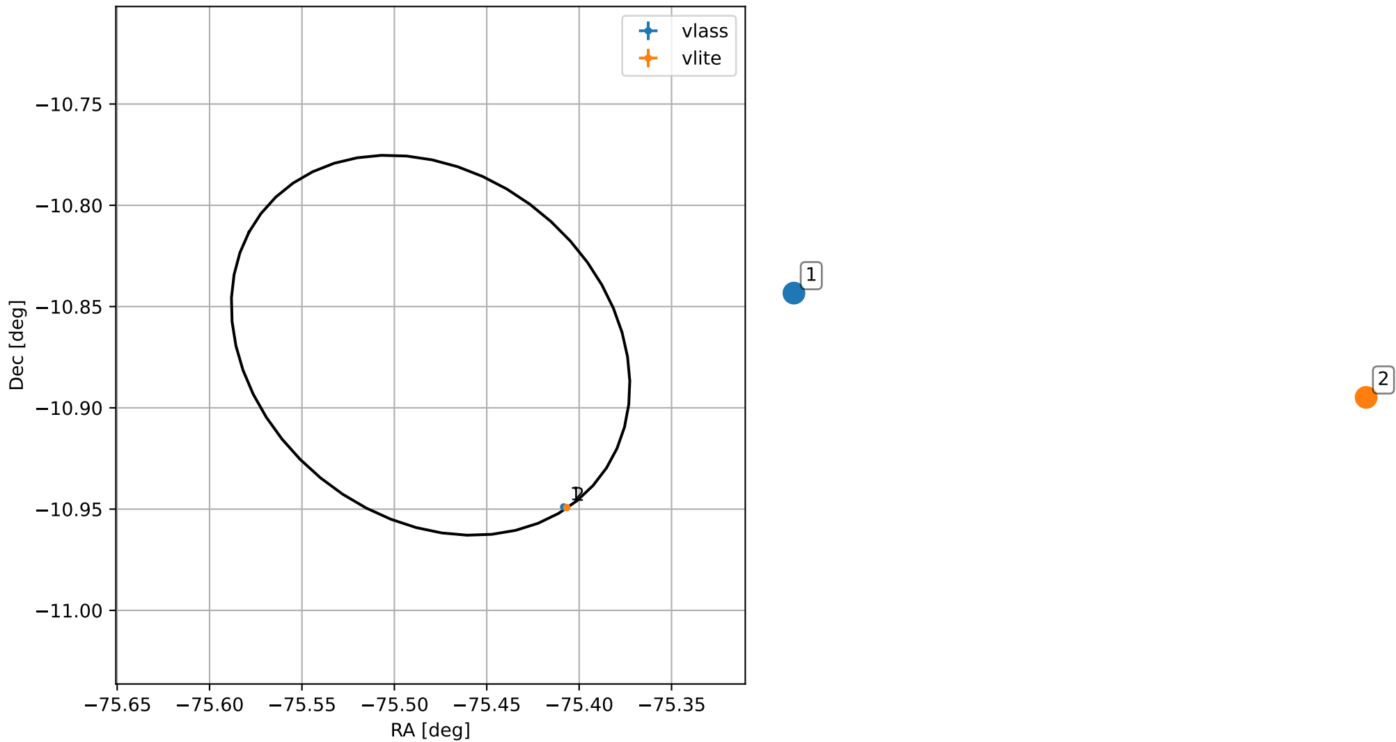
4FGL J1858.0-1052
