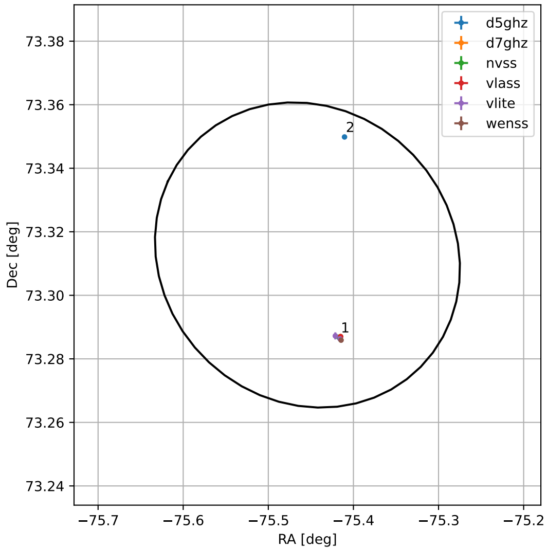
4FGL J1858.1+7318
