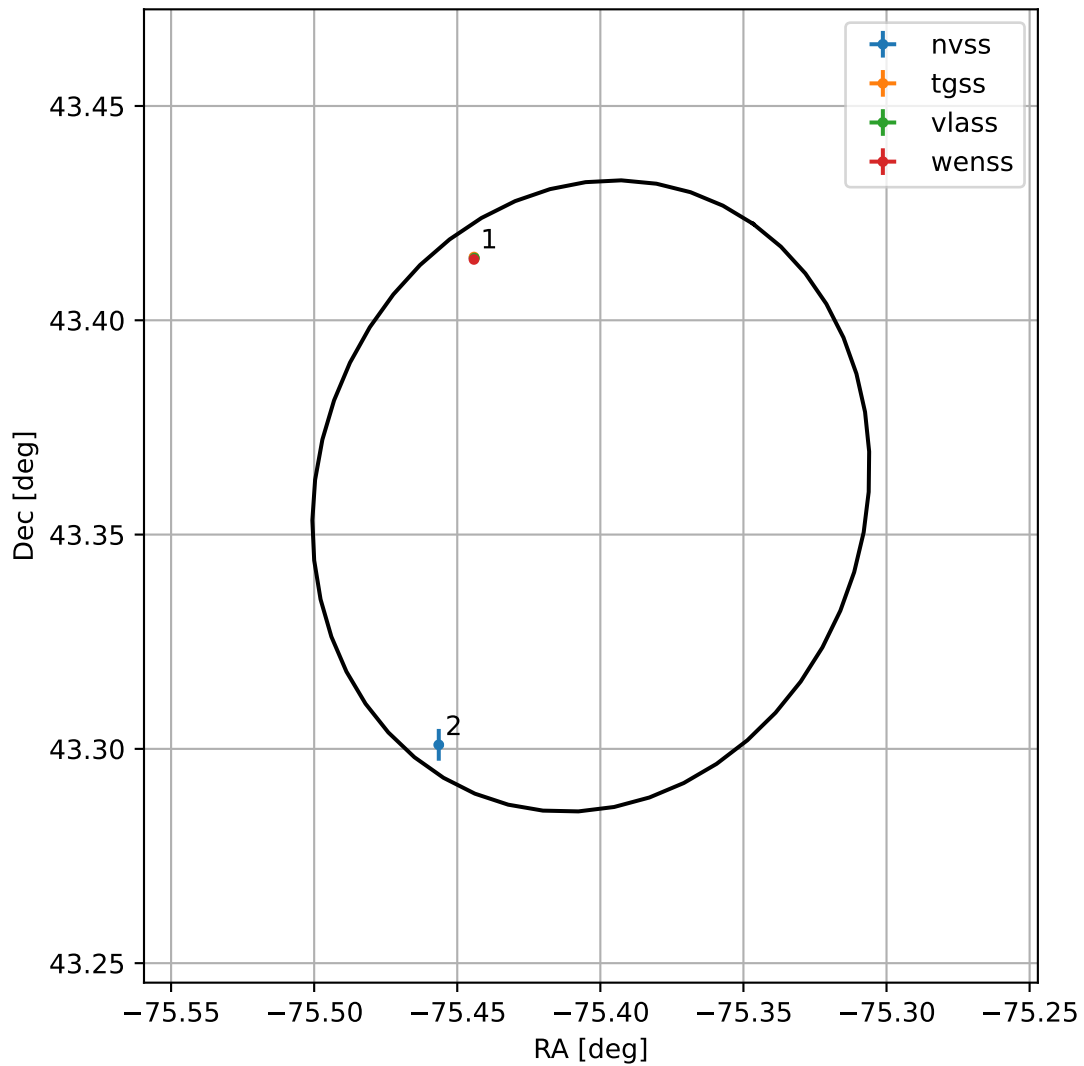
4FGL J1858.3+4321
