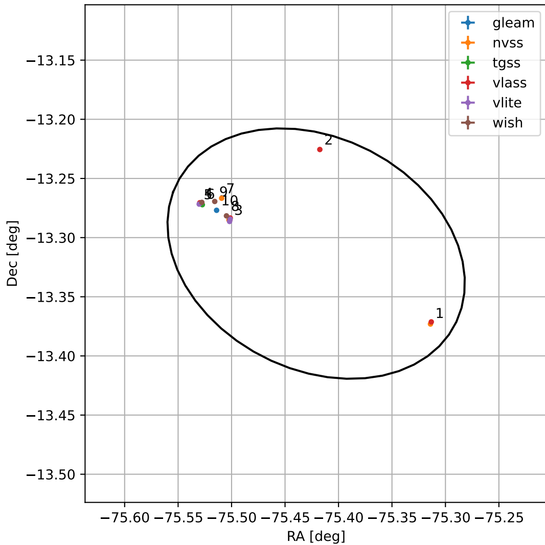
4FGL J1858.3-1318
