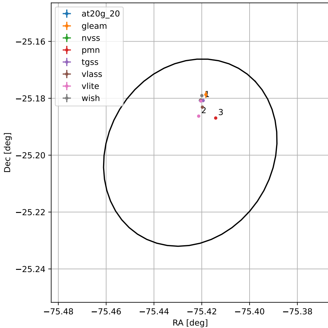
4FGL J1858.3-2511
