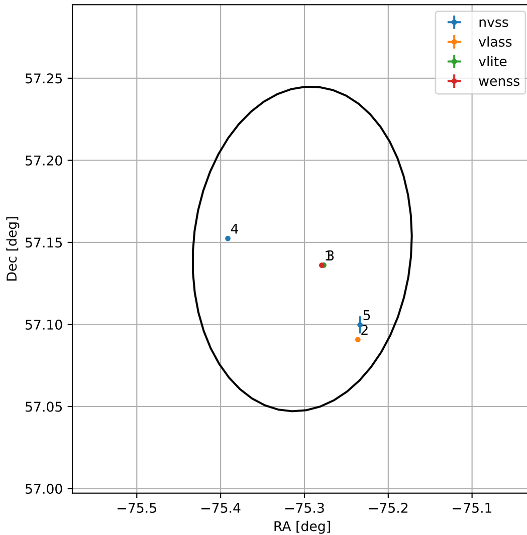
4FGL J1858.7+5708
