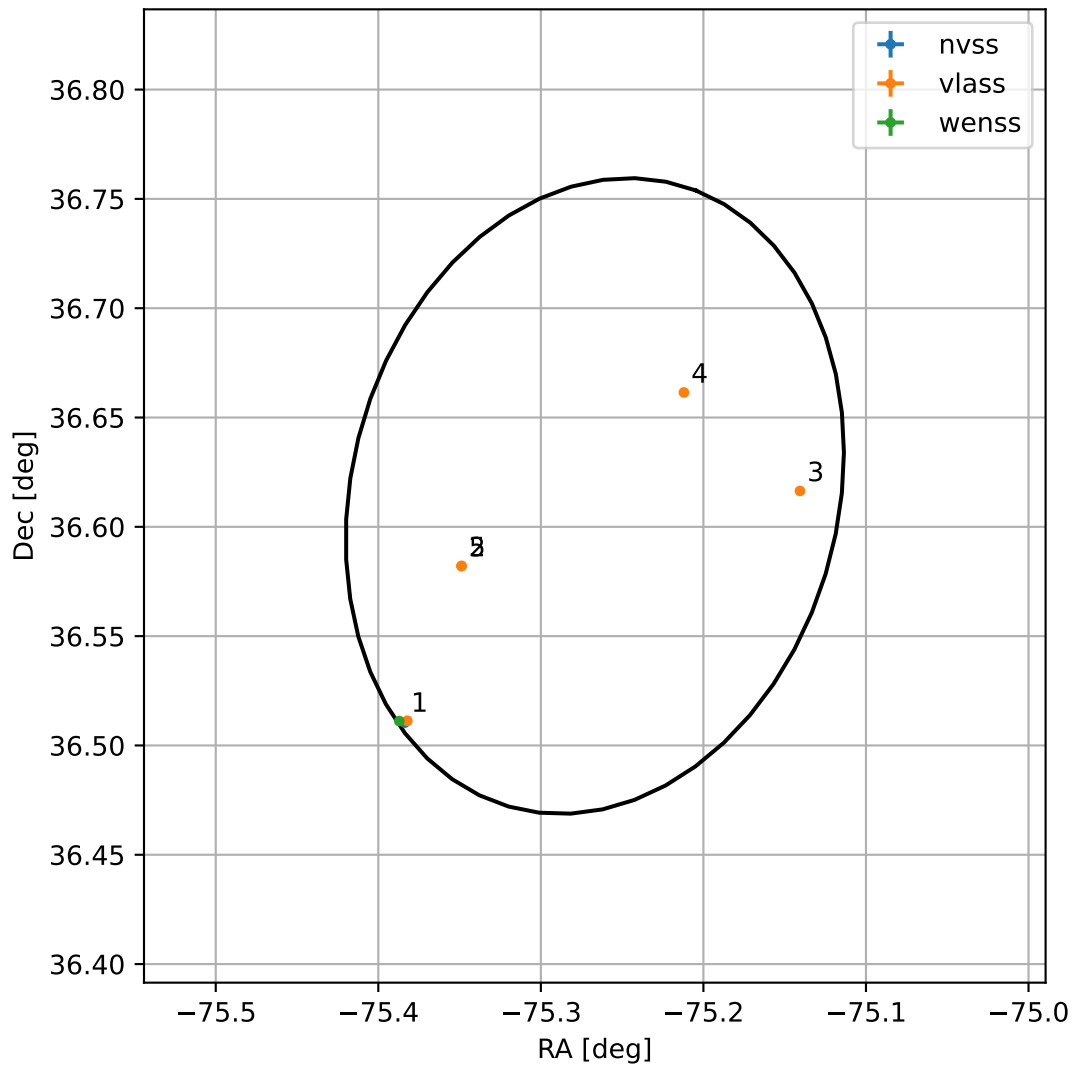
4FGL J1858.9+3636
