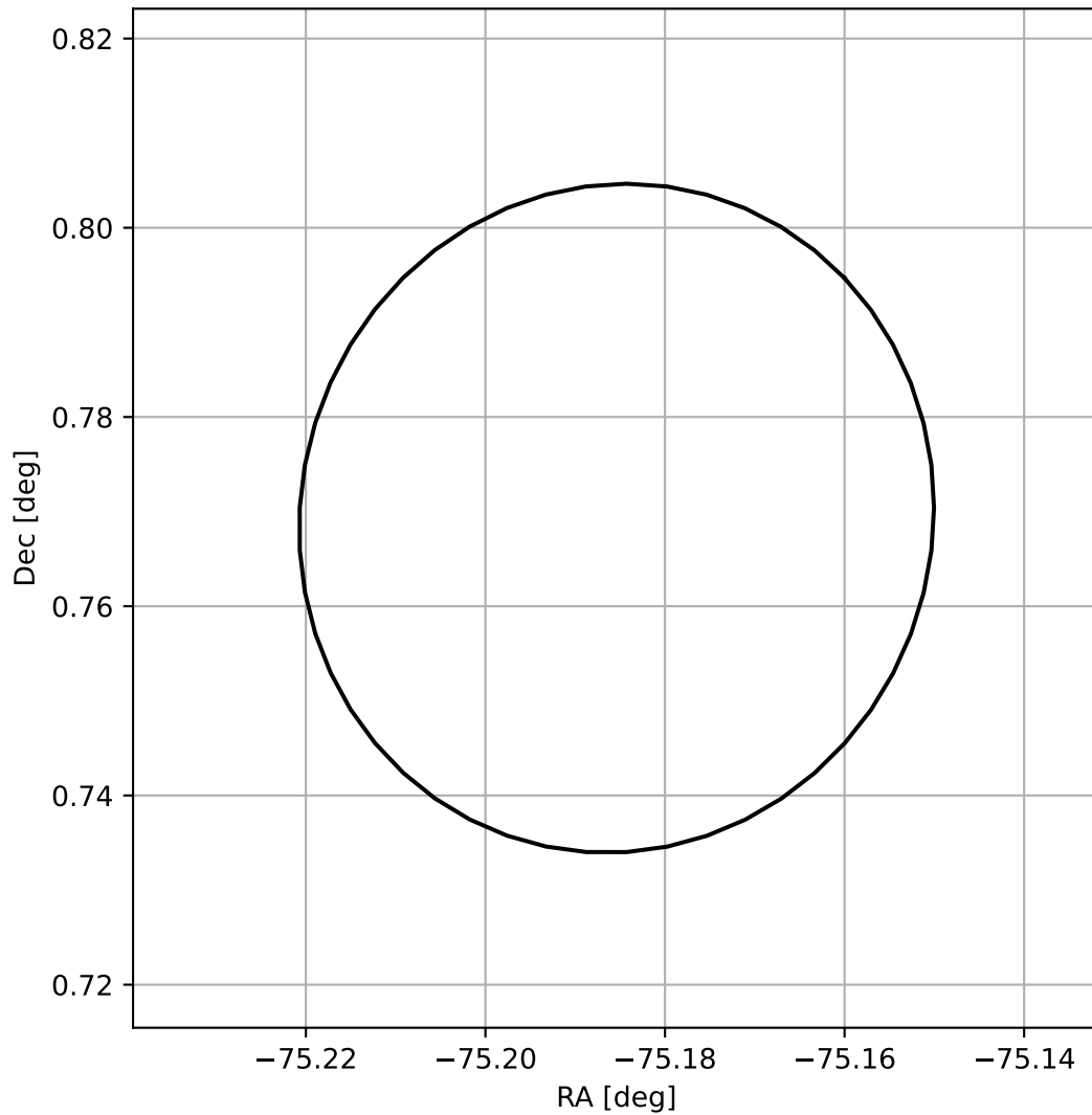
4FGL J1859.2+0046
