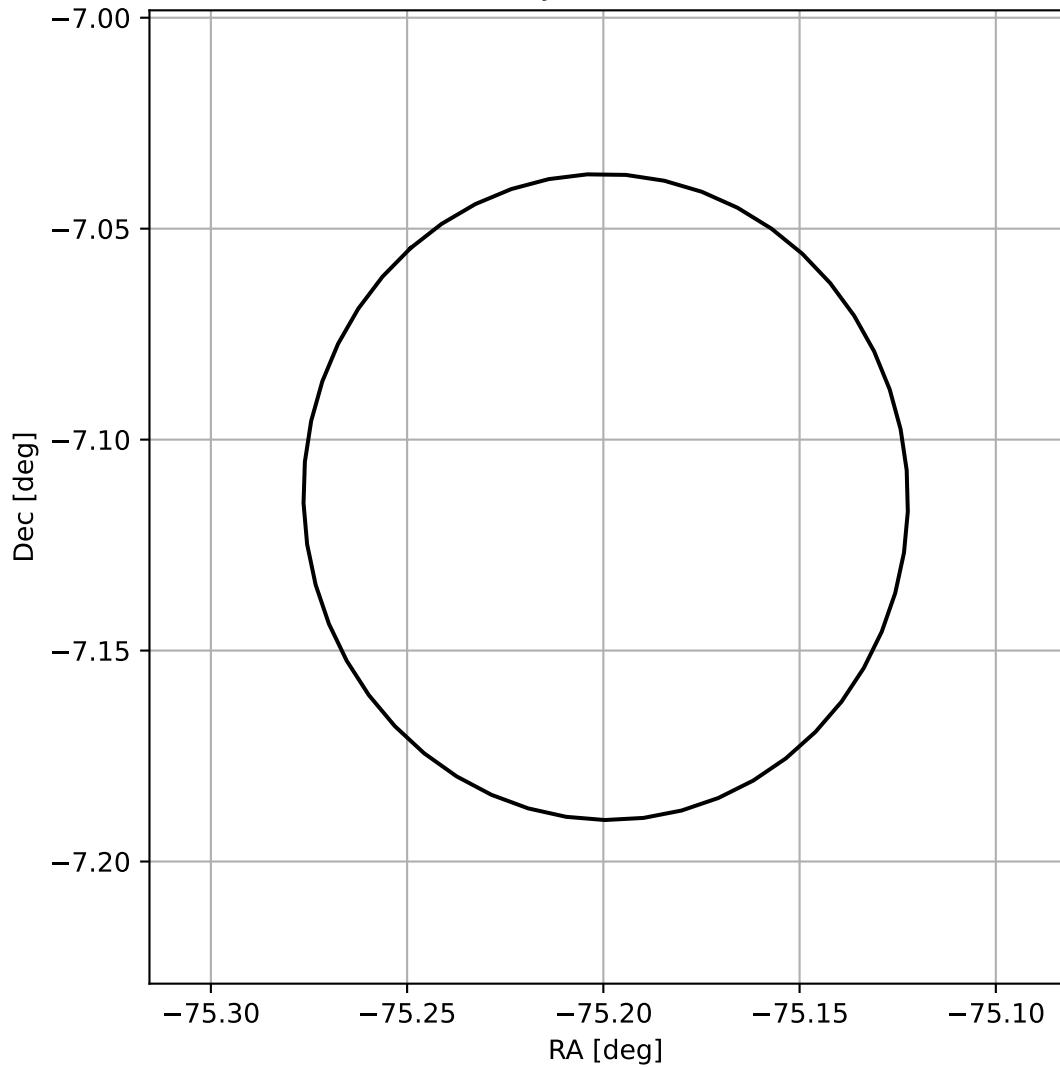
4FGL J1859.2-0706
