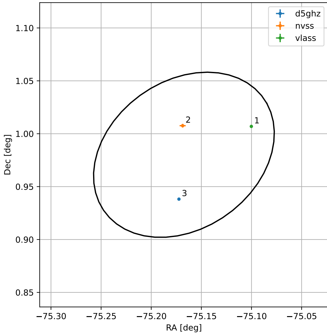
4FGL J1859.3+0058
