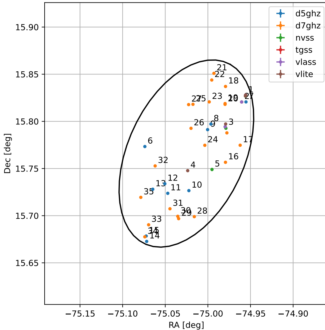
4FGL J1859.8+1545
