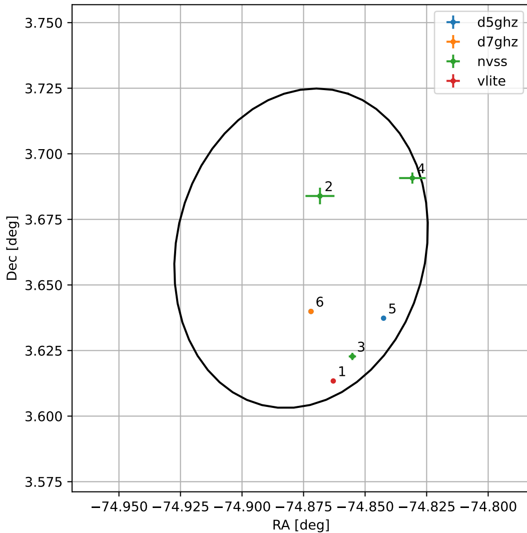
4FGL J1900.4+0339
