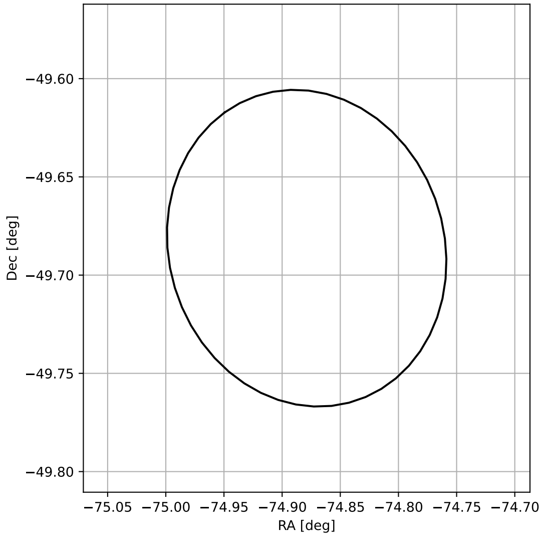
4FGL J1900.4-4941
