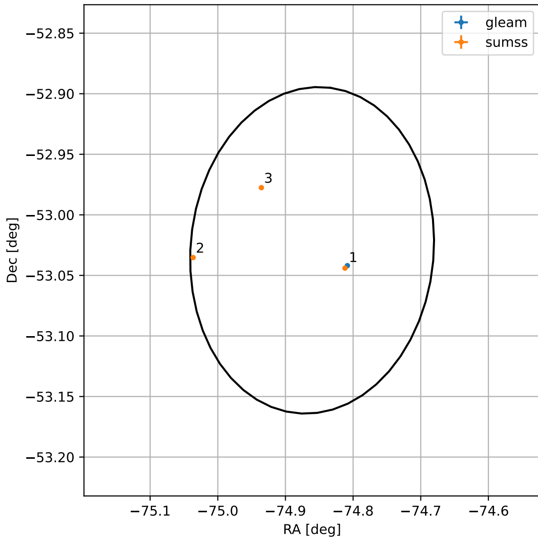
4FGL J1900.5-5301
