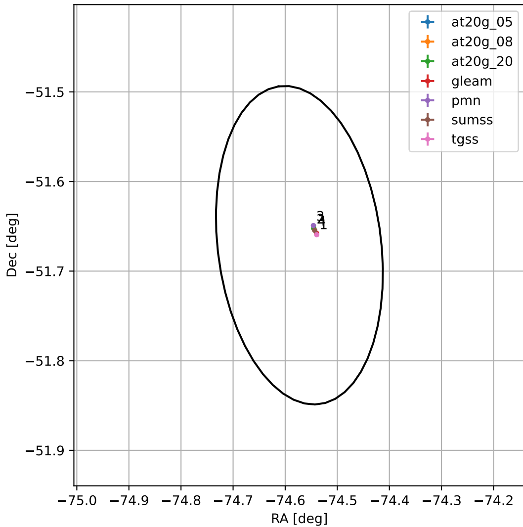
4FGL J1901.7-5140
