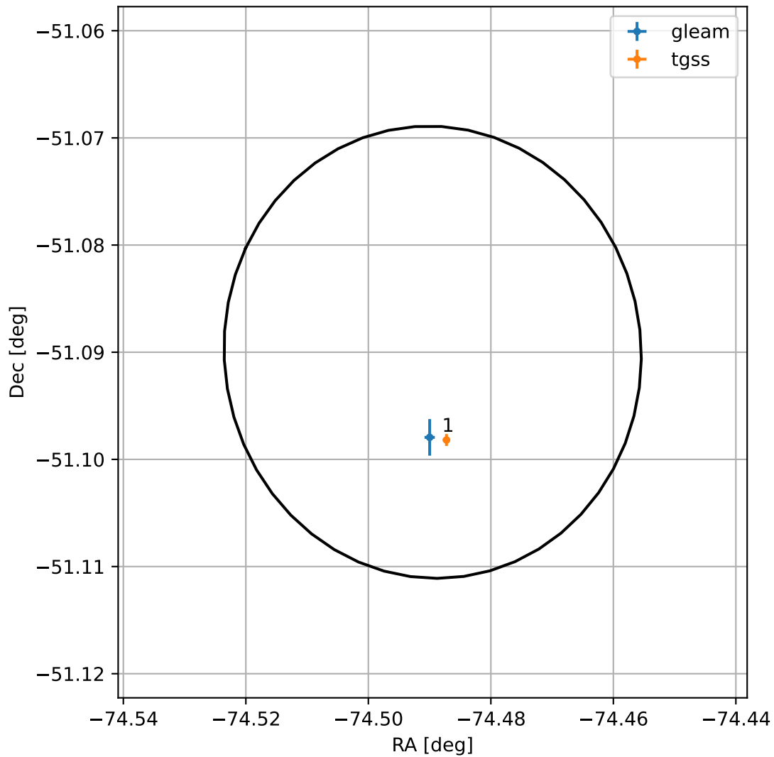
4FGL J1902.0-5105
