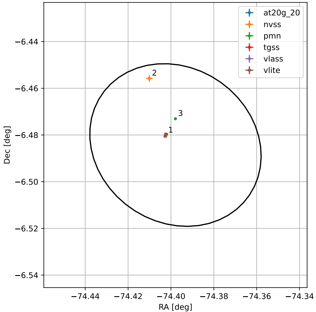
4FGL J1902.4-0629
