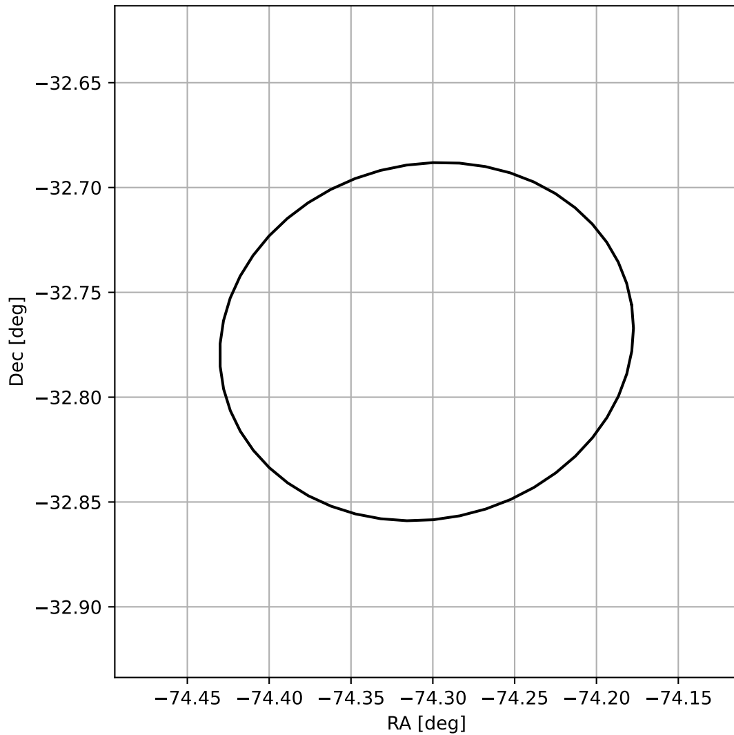
4FGL J1902.7-3246
