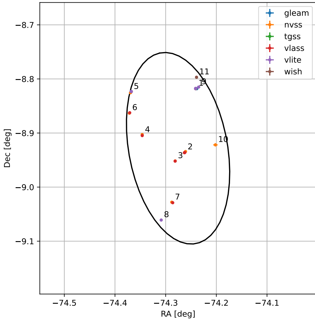
4FGL J1902.8-0855
