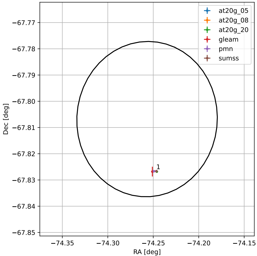
4FGL J1902.9-6748
