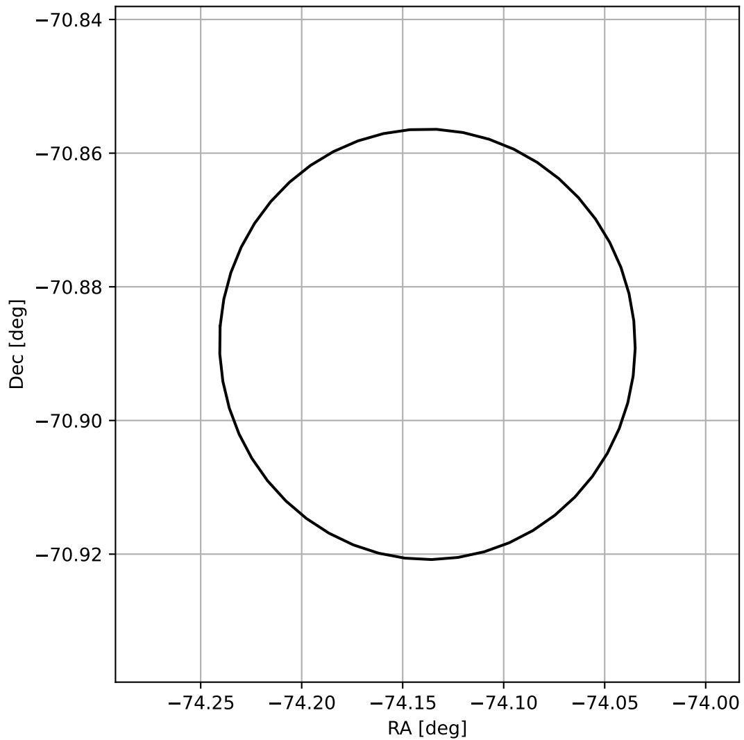
4FGL J1903.4-7053
