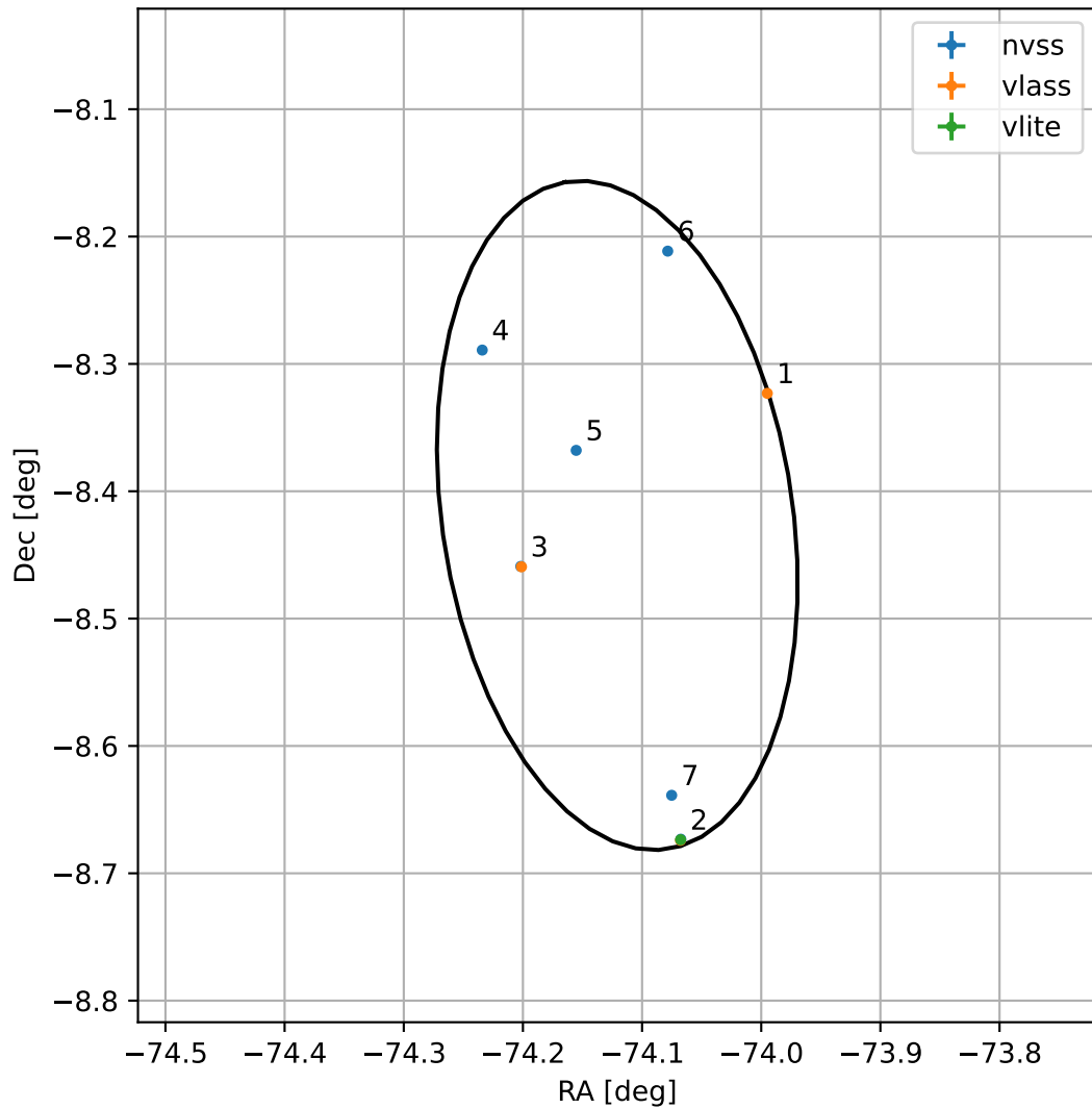
4FGL J1903.5-0825
