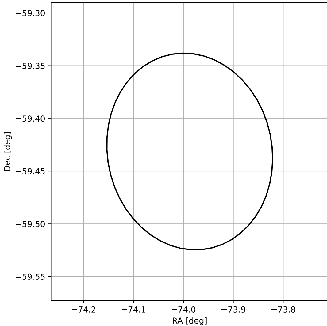
4FGL J1904.0-5925
