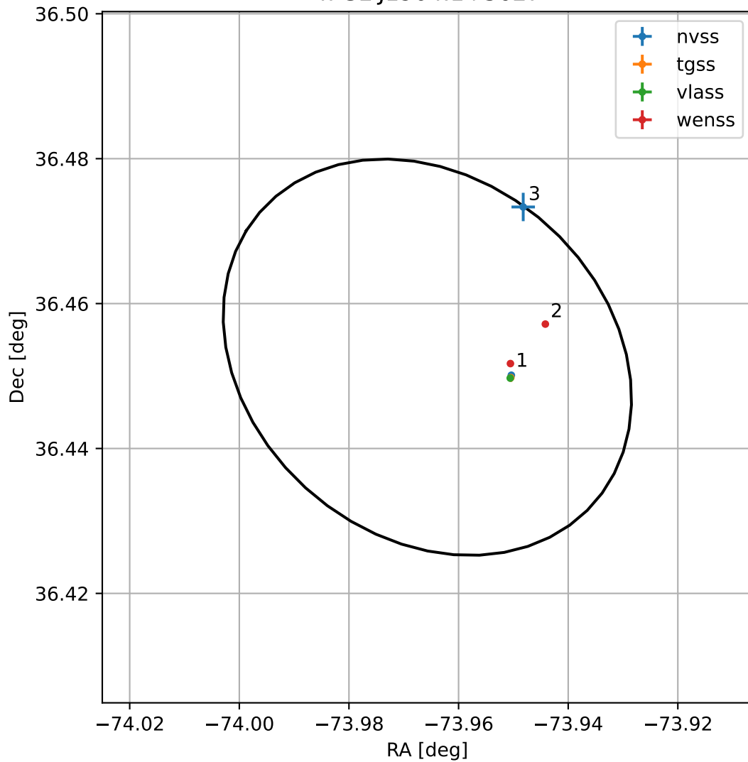
4FGL J1904.1+3627
