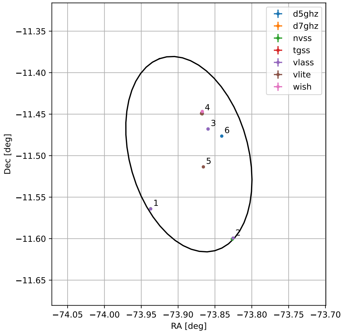
4FGL J1904.4-1129
