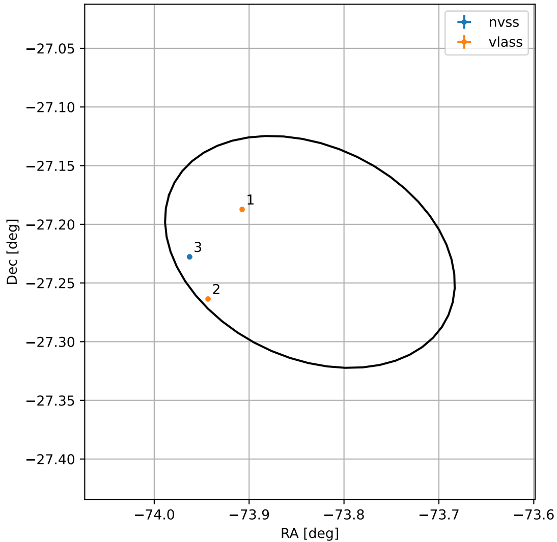
4FGL J1904.6-2713
