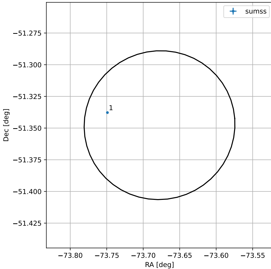
4FGL J1905.2-5120
