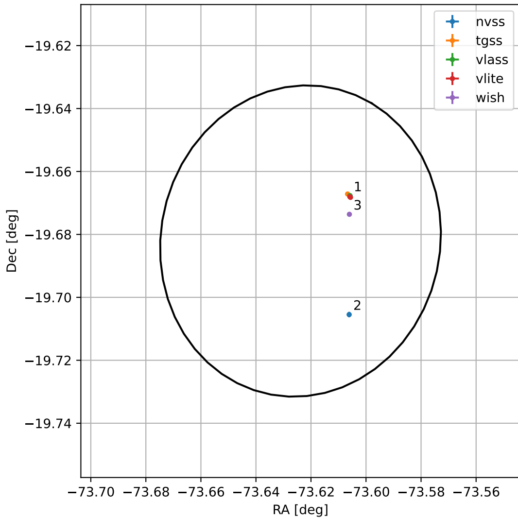
4FGL J1905.5-1940
