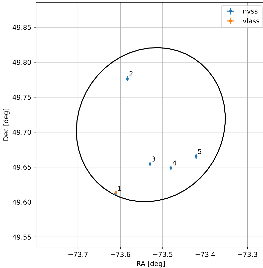
4FGL J1905.8+4942
