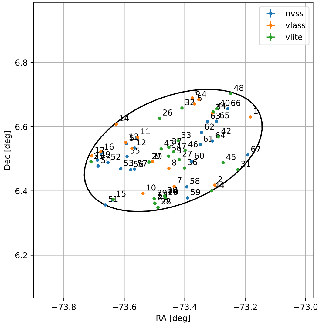
4FGL J1906.2+0631
