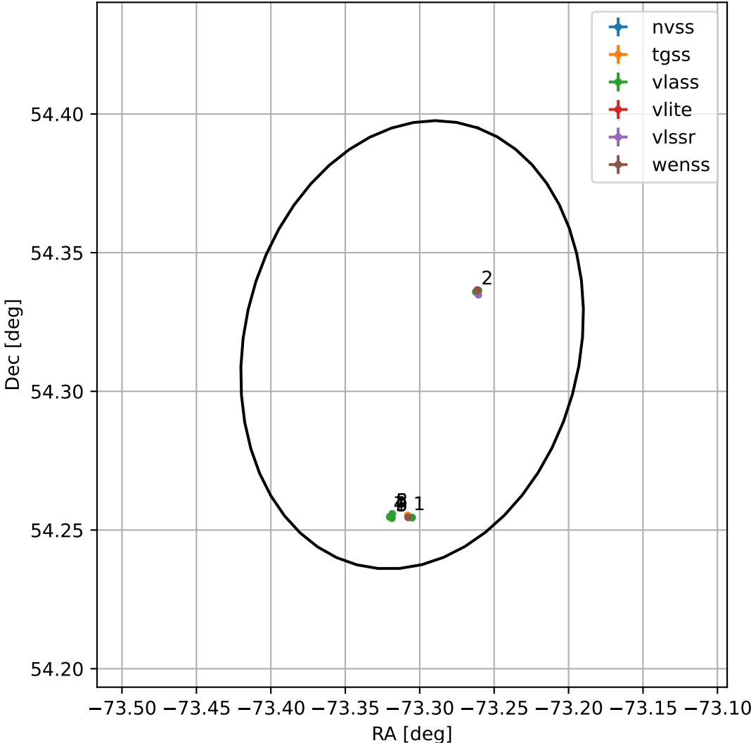
4FGL J1906.7+5419
