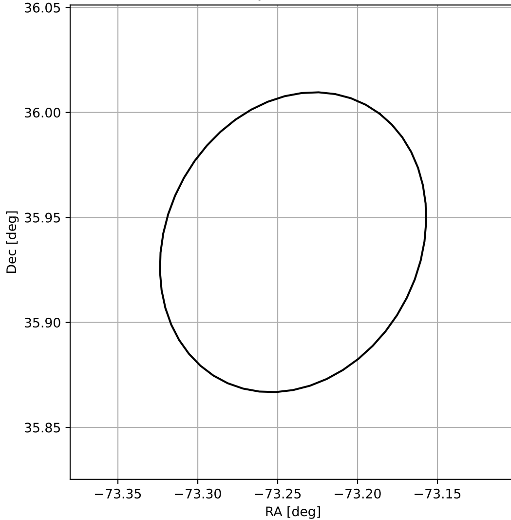
4FGL J1907.0+3556
