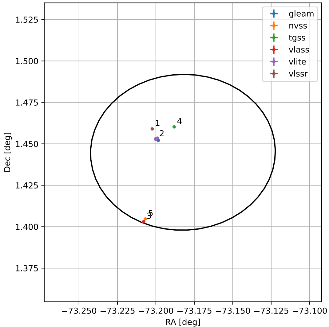
4FGL J1907.2+0126
