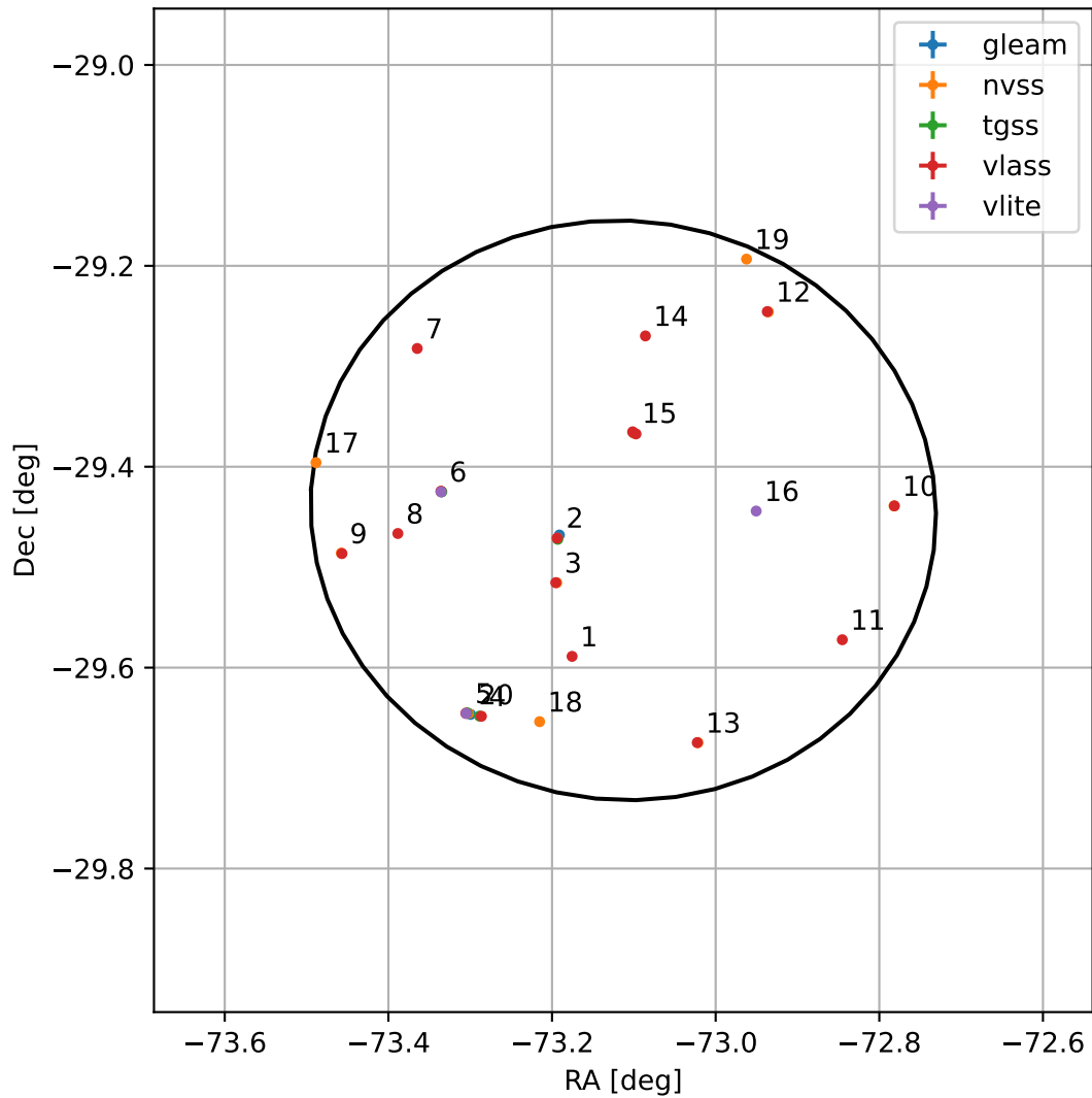
4FGL J1907.5-2926
