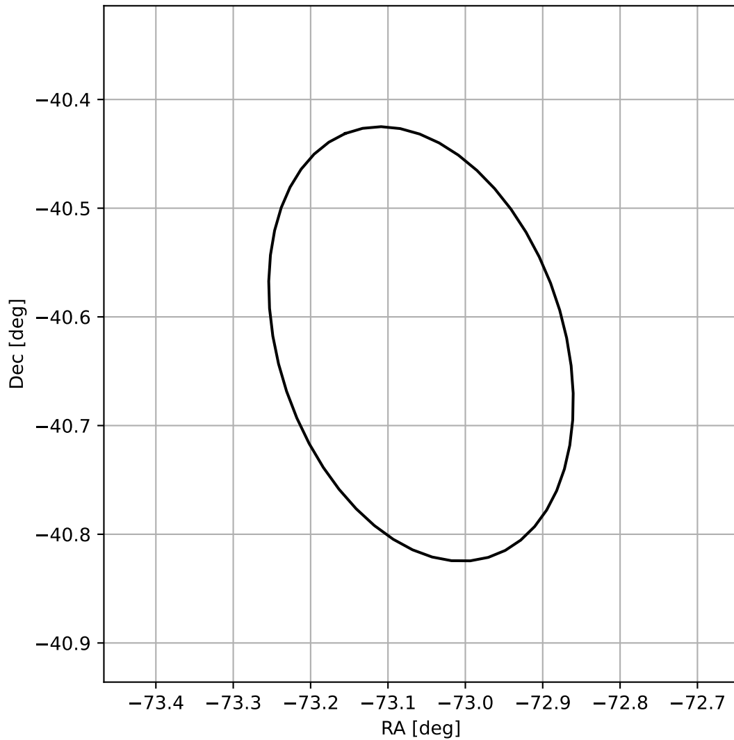
4FGL J1907.7-4037
