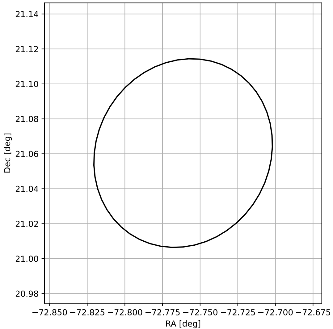
4FGL J1908.9+2103
