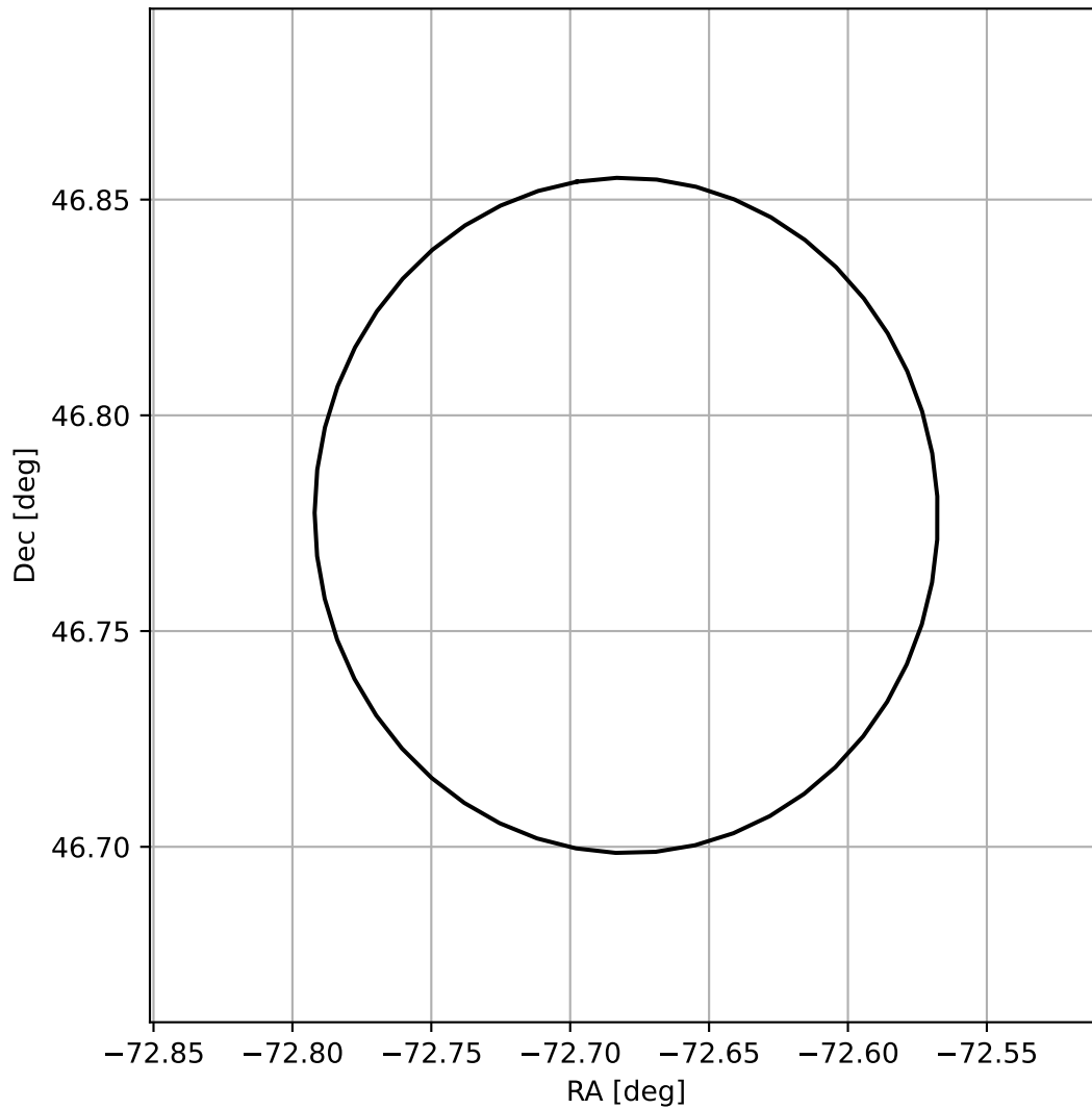
4FGL J1909.2+4646
