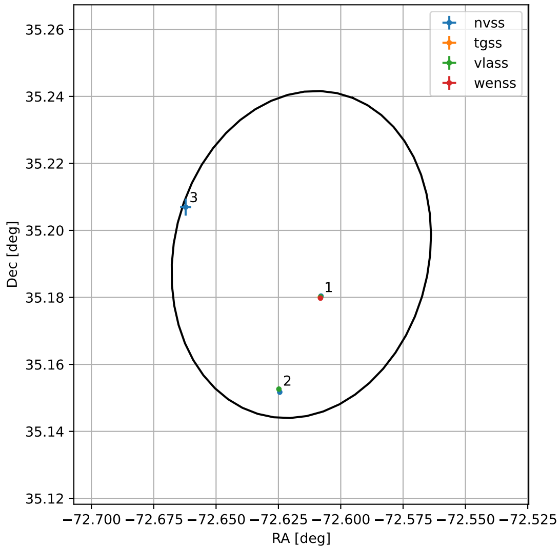
4FGL J1909.5+3511
