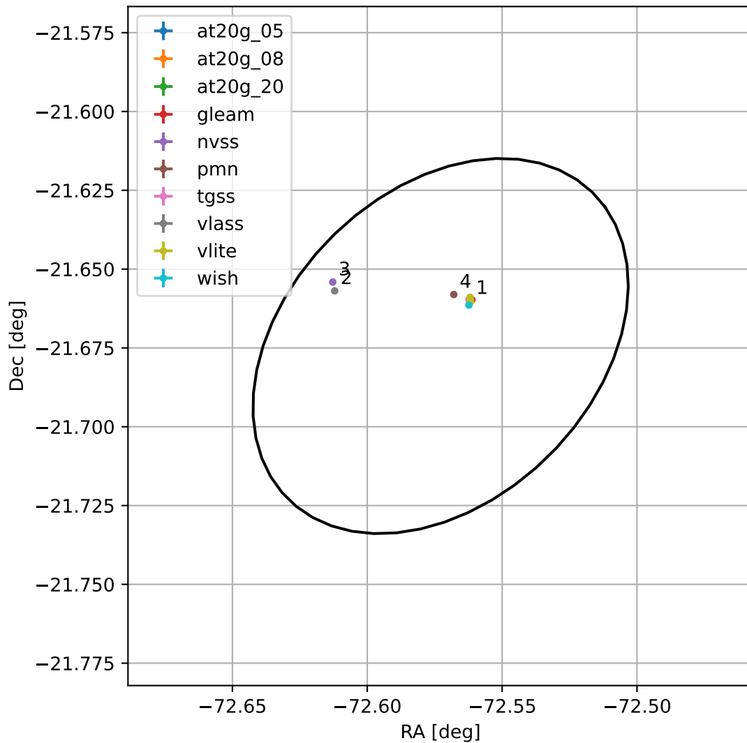
4FGL J1909.7-2140
